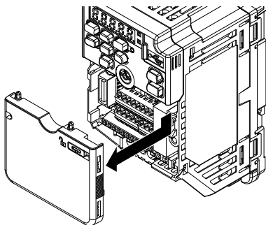
Figure 5.30 Remove the Front Cover
