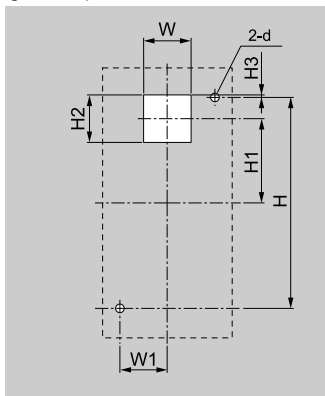
Figure 5.9 External/Face Mount Enclosure Panel Cut-Out Dimensions
