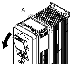
Figure 5.40 Removing the Included Drive Keypad
