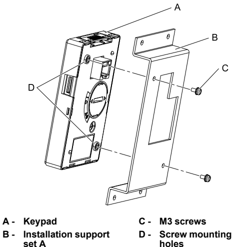
Figure 5.38 Mounting the Keypad to Installation Support Set A
