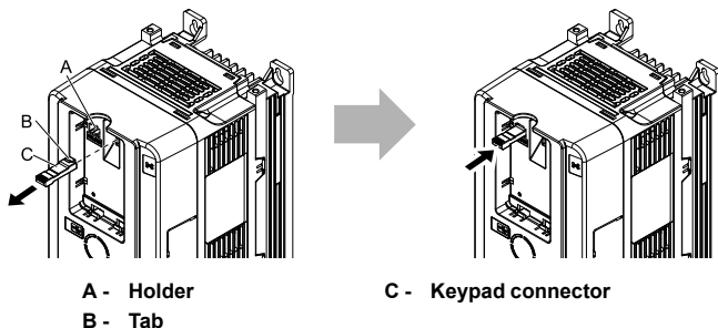
Figure 5.12 Moving the Keypad Connector to the Holder
