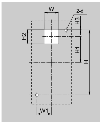
Figure 5.33 External/Face Mount Enclosure Panel Cut-Out Dimensions
