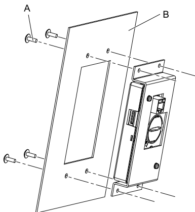
Figure 5.28 Internal/Flush-Mount Installation
