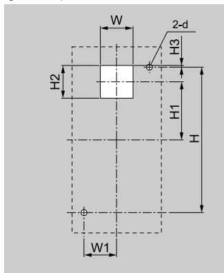
Figure 5.20 External/Face Mount Enclosure Panel Cut-Out Dimensions
