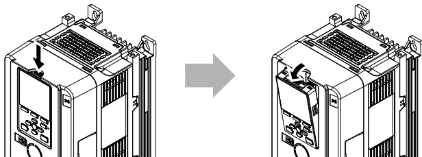
Figure 5.17 Removing the Included Drive Keypad
