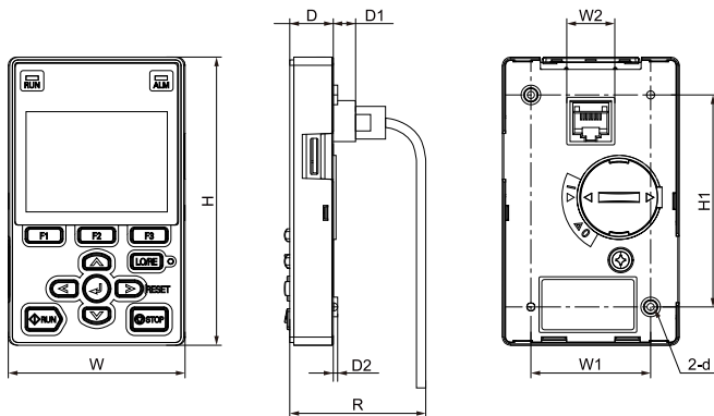
Figure 5.8 Exterior and Mounting Dimensions
