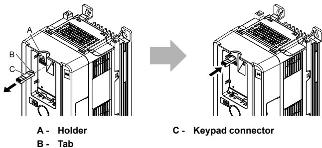
Figure 5.18 Moving the Keypad Connector to the Holder
