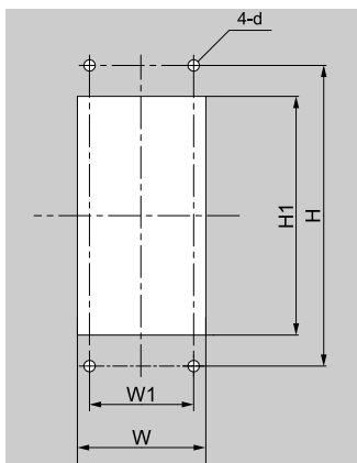
Figure 5.26 Internal/Flush-Mount Enclosure Panel Cut-Out Dimensions
