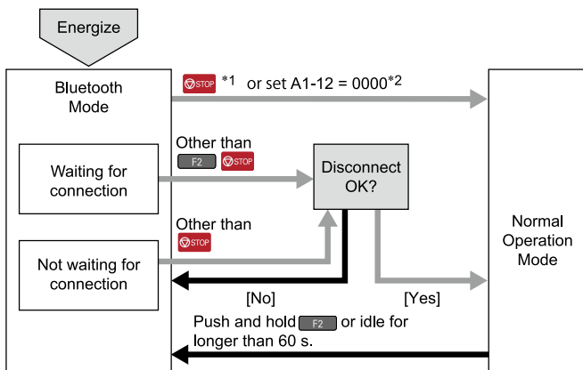
Figure 5.7 Changing between Bluetooth Mode and Normal Operation Mode
