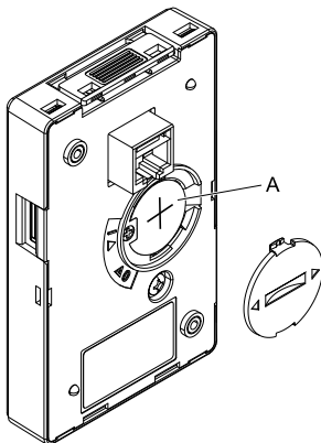
Figure 5.43 Insert the New Battery
